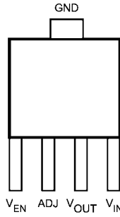
20126803 SOT-223, Top View LP38693MP-ADJ
